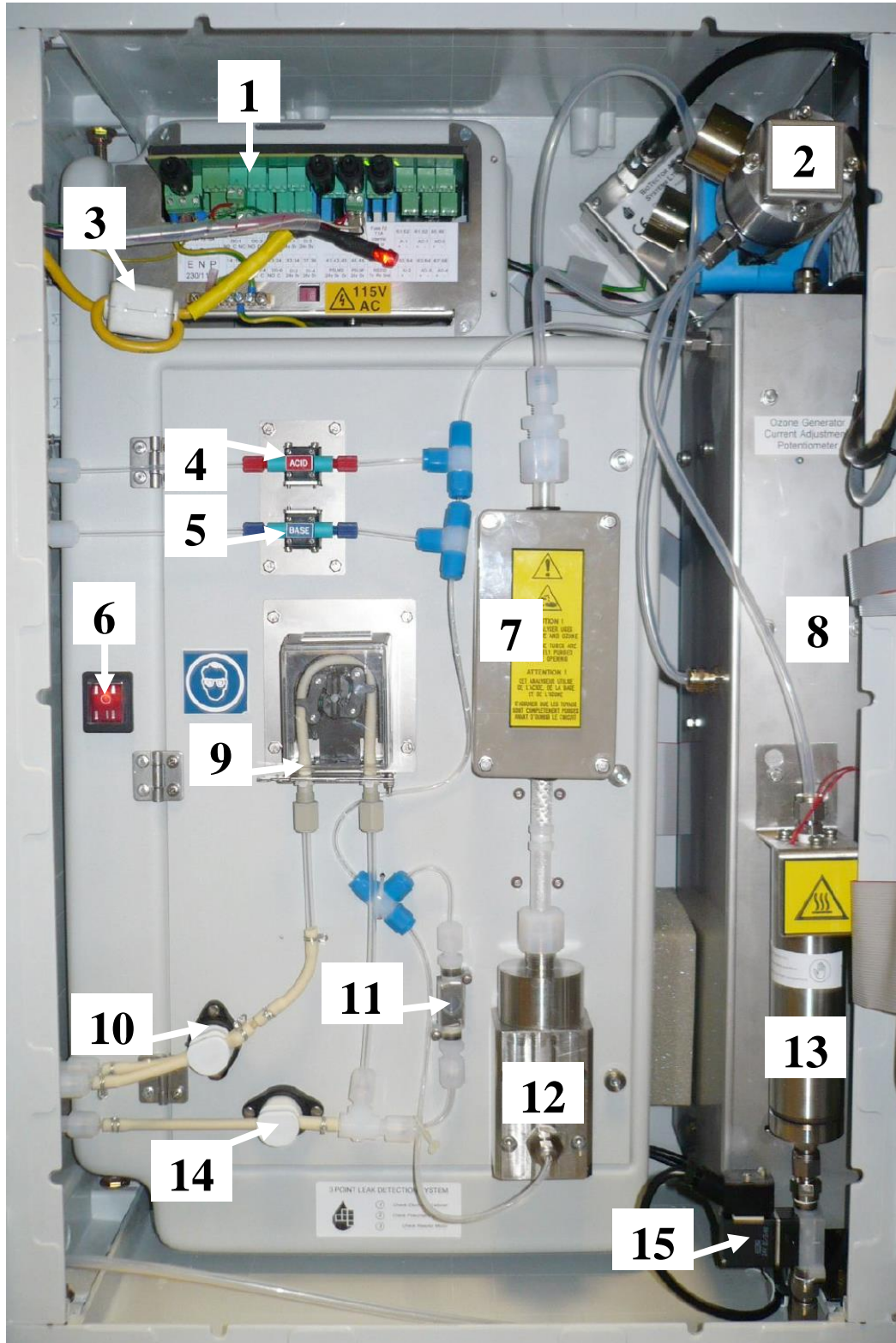
Figure 1 BioTector analysis enclosure major components (typical TIC & TOC system)
