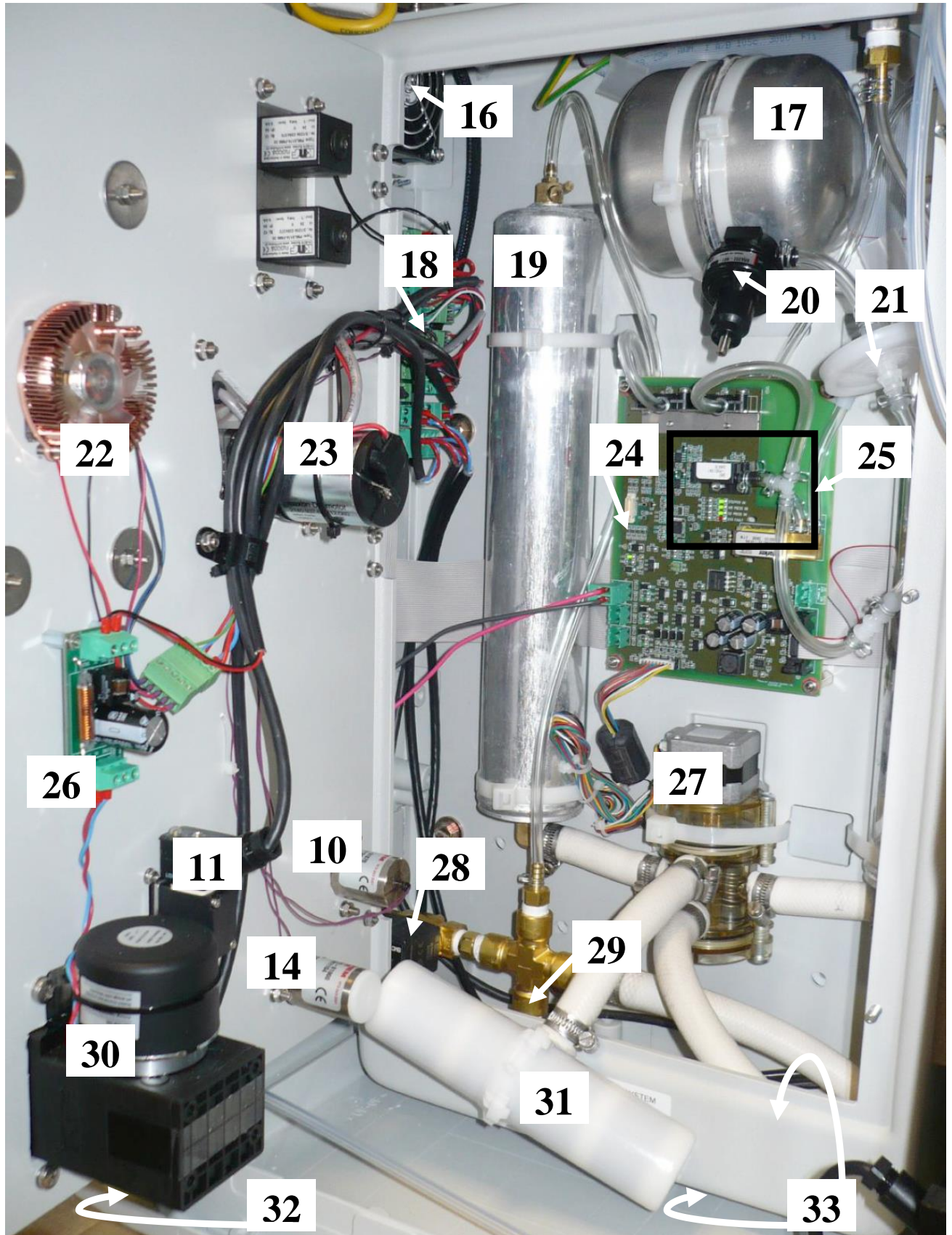
Figure 2 BioTector oxygen concentrator enclosure major components
