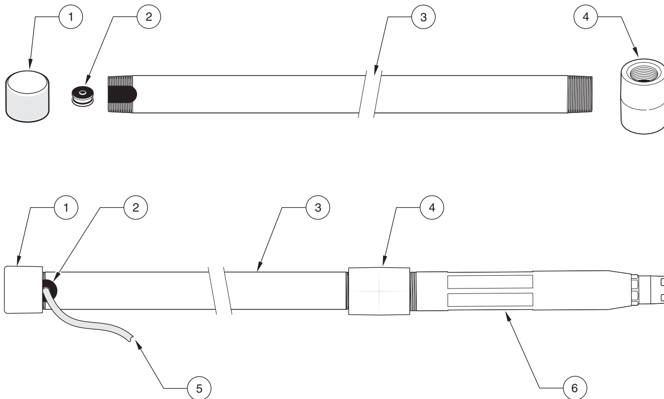
Figure 1 pH Immersion Mounting Components and Final Assembly
